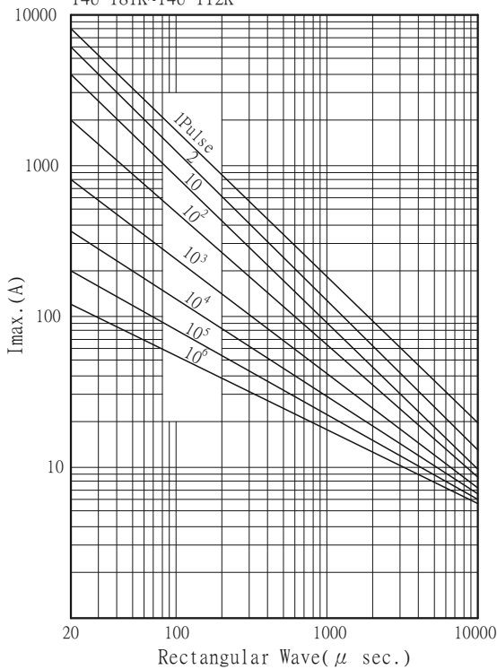
Pulse Life time Ratings - 14mm 14U 181K~14U 112K
