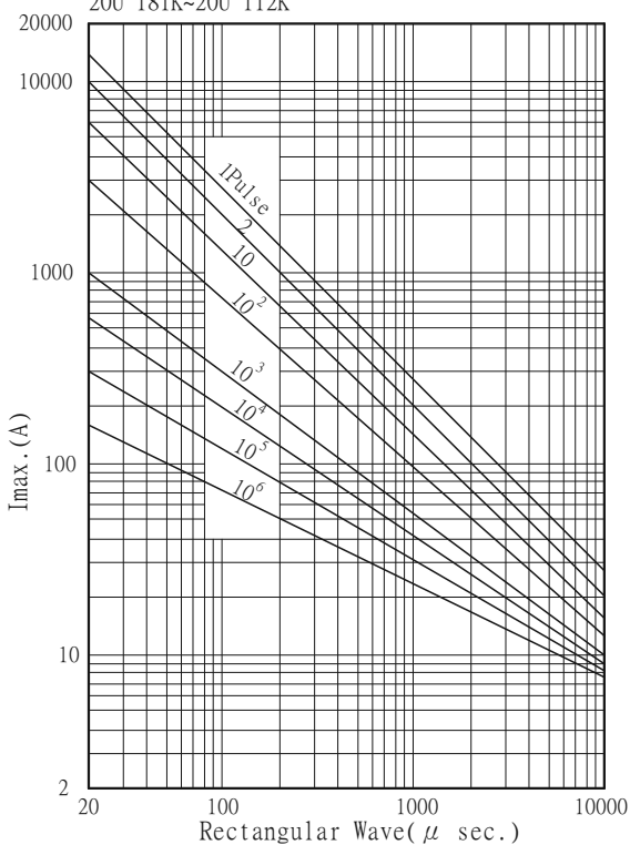
Pulse Life time Ratings -20mm 20U 181K~20U 112K
