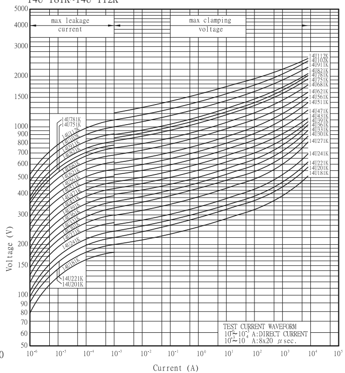
V-I Characteristic Curve - 14mm 14U 181K~14U 112K
