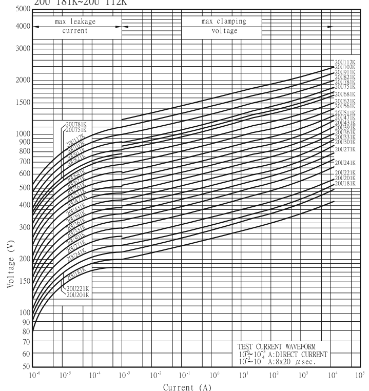
V-I Characteristic Curve -20mm 20U 181K~20U 112K
