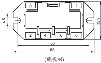
HF116F-1/□□□□-□-F-1H-□
